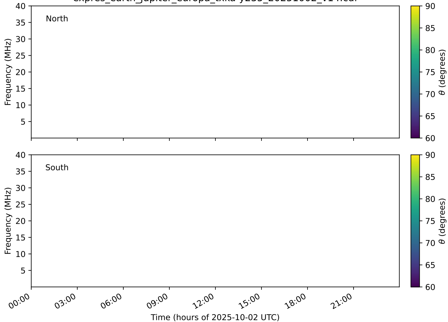
expres_earth_jupiter_europa_txka-y235_20251002_v14.cdf
