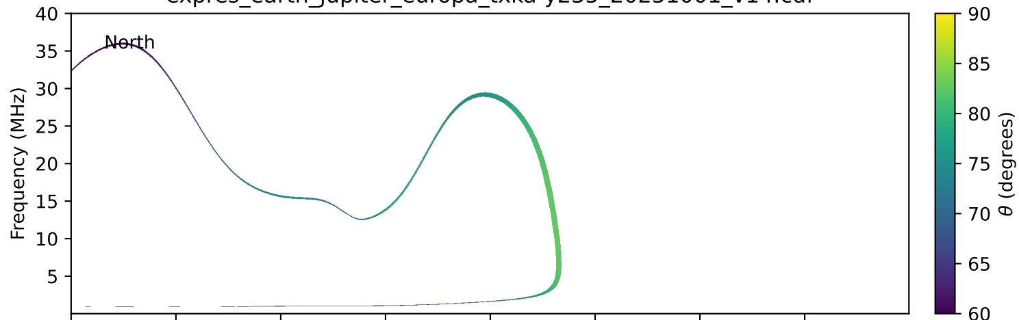
expres_earth_jupiter_europa_txka-y235_20251001_v14.cdf
