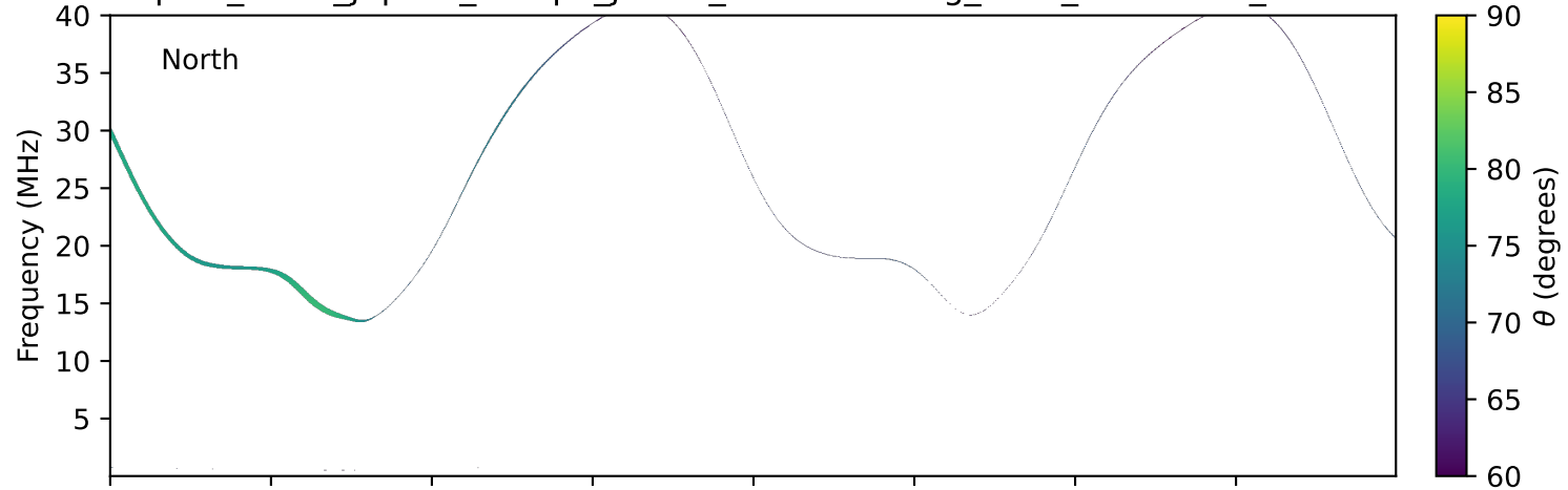
expres_earth_jupiter_europa_jrm33_lossc-wid1deg_3kev_20251025_v11.cdf
