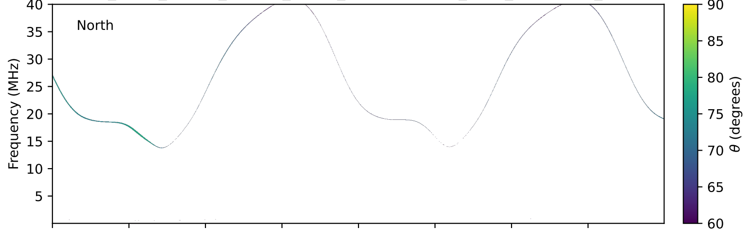
expres_earth_jupiter_europa_jrm33_lossc-wid1deg_3kev_20251018_v11.cdf
