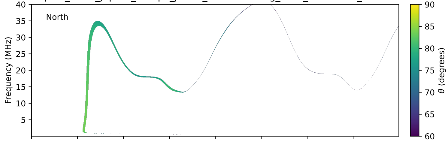
expres_earth_jupiter_europa_jrm33_lossc-wid1deg_3kev_20251007_v11.cdf
