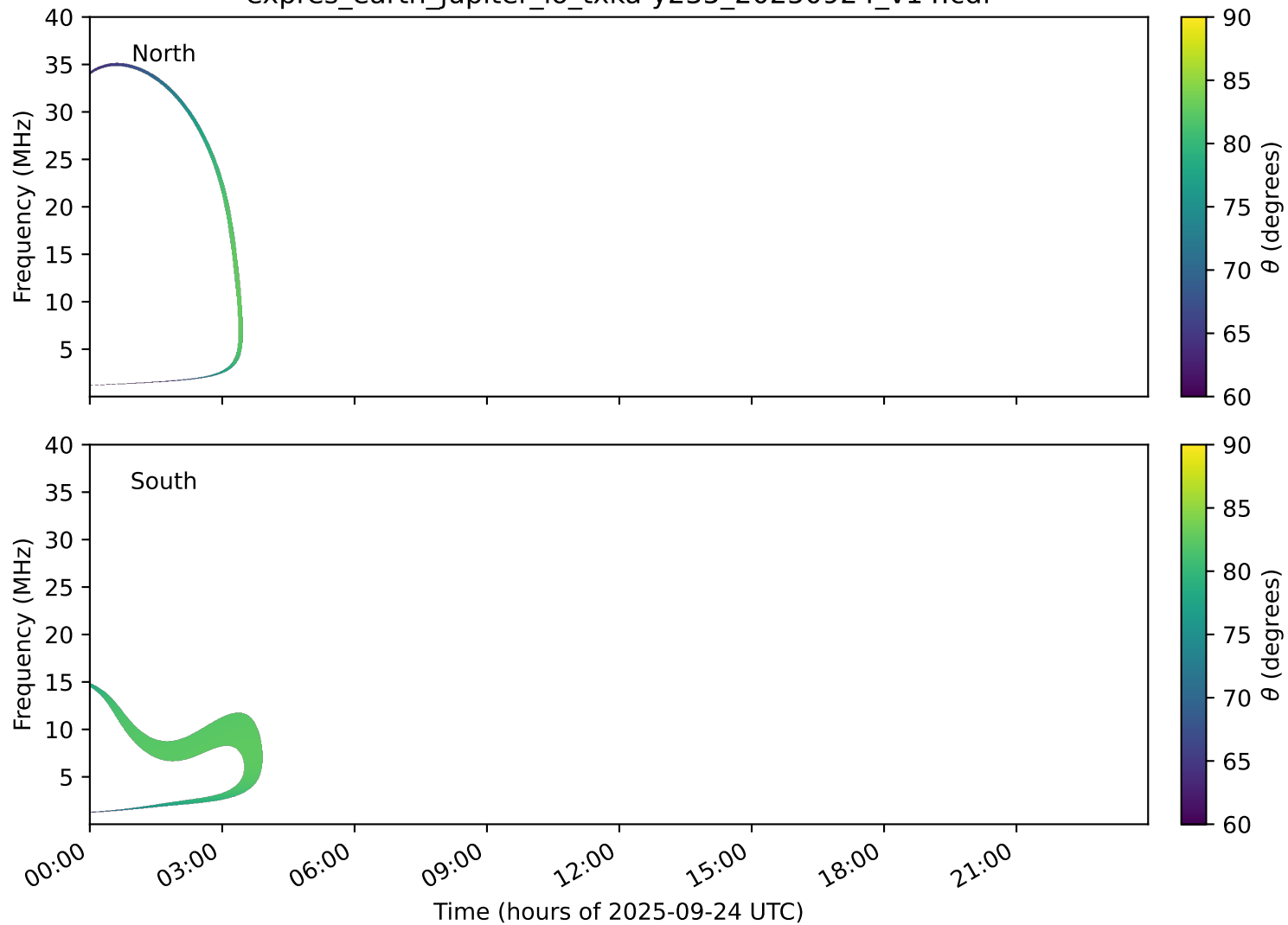
expres_earth_jupiter_io_txka-y235_20250924_v14.cdf
