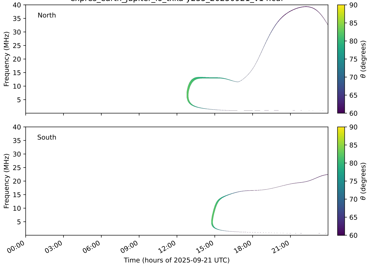
expres_earth_jupiter_io_txka-y235_20250921_v14.cdf
