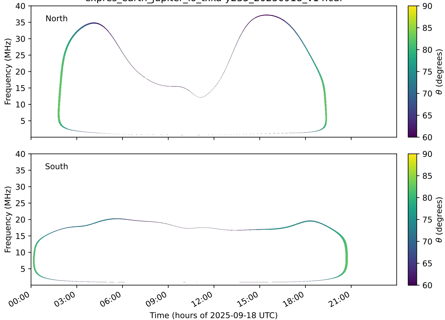
expres_earth_jupiter_io_txka-y235_20250918_v14.cdf
