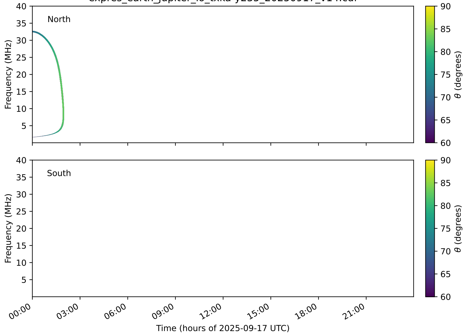
expres_earth_jupiter_io_txka-y235_20250917_v14.cdf
