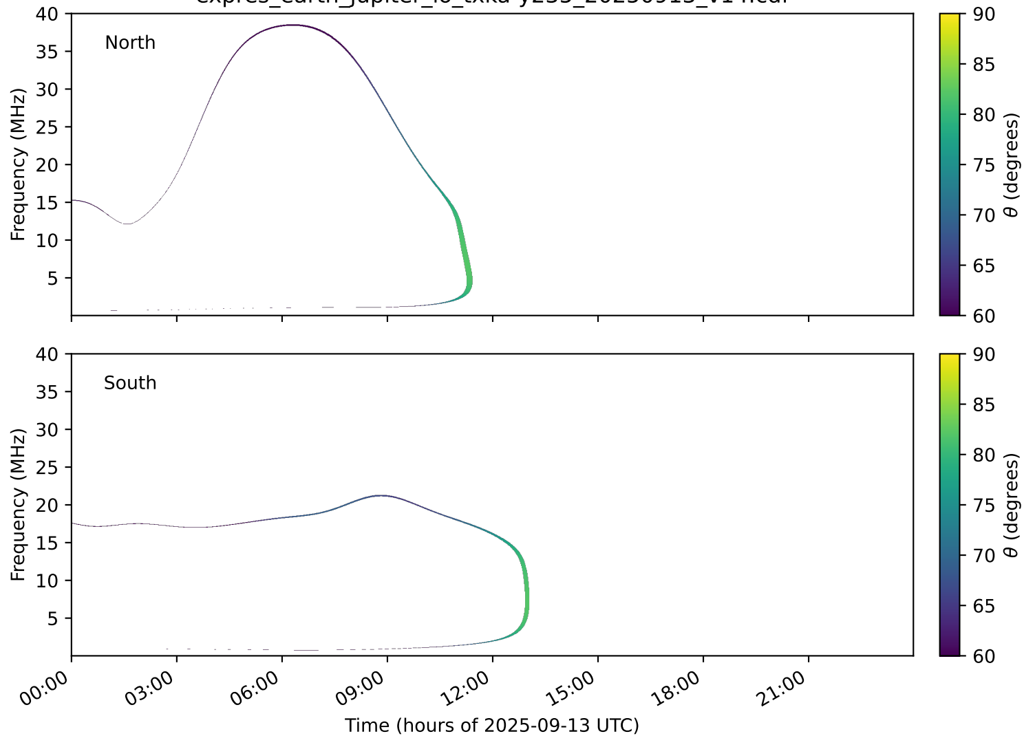
expres_earth_jupiter_io_txka-y235_20250913_v14.cdf
