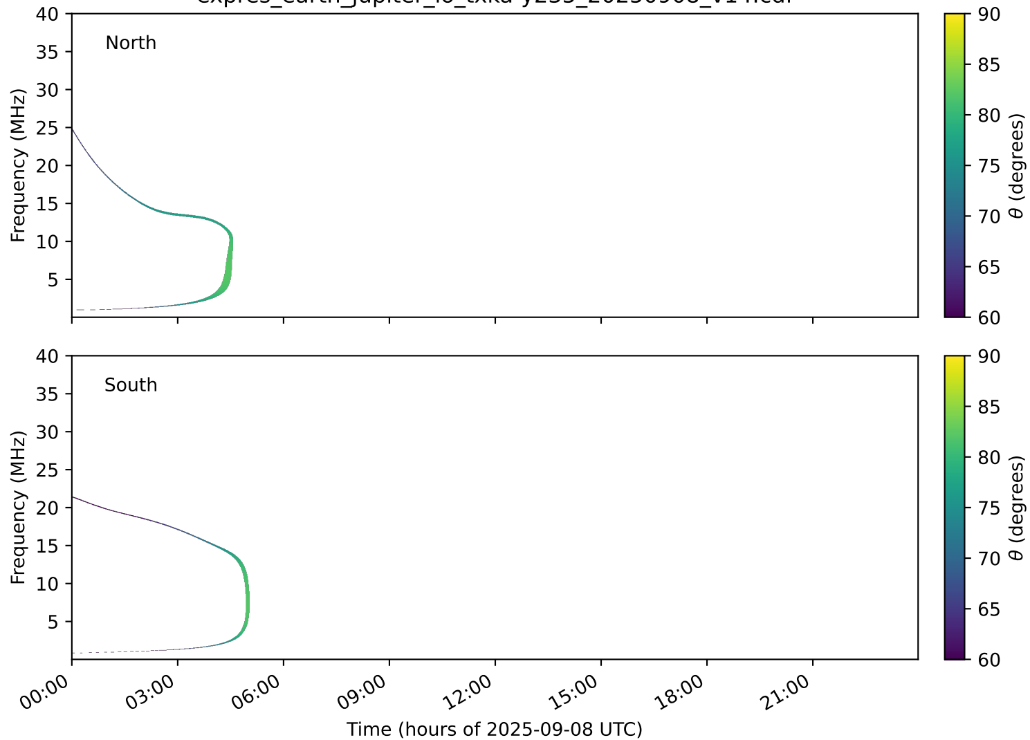
expres_earth_jupiter_io_txka-y235_20250908_v14.cdf
