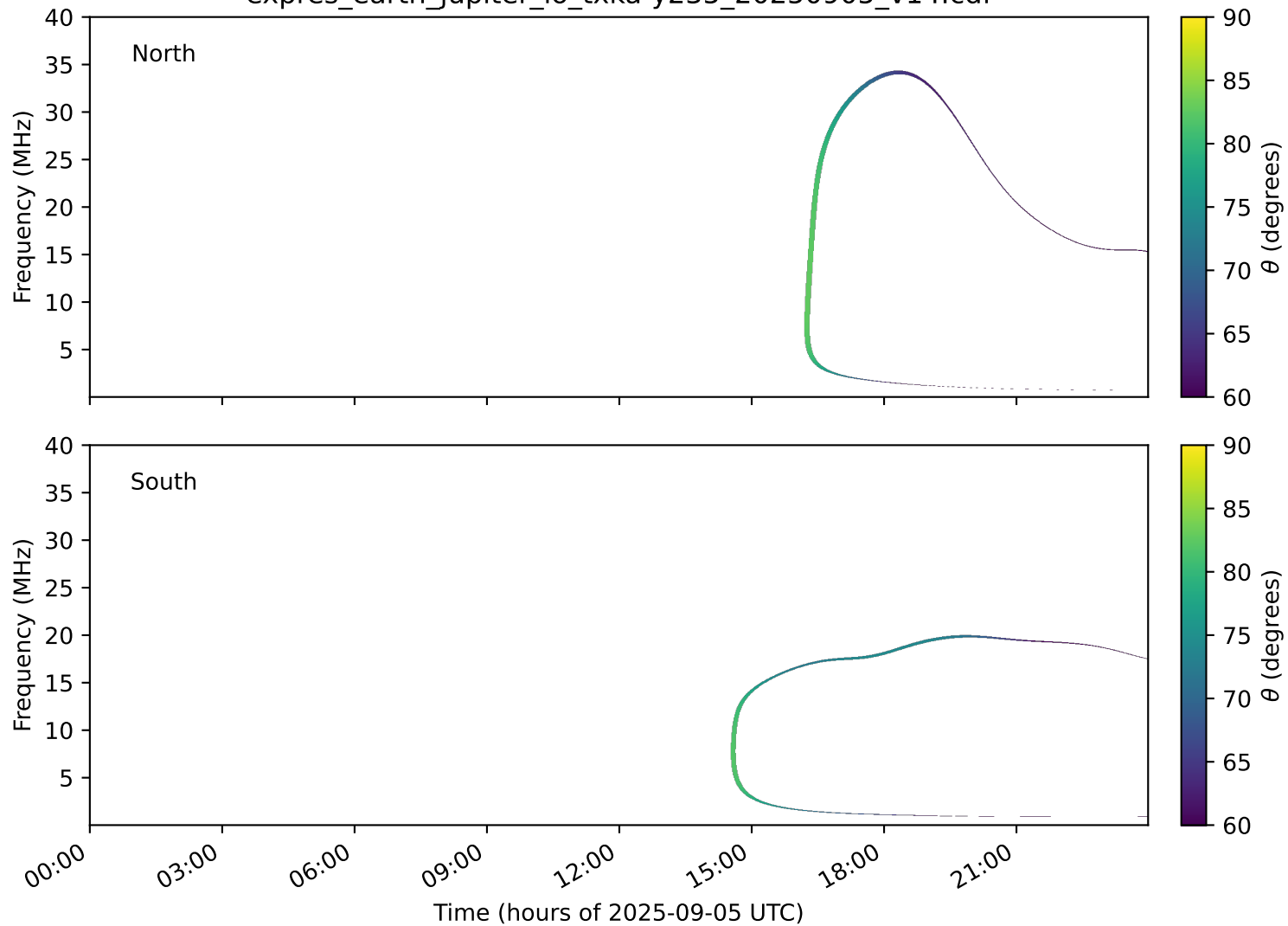
expres_earth_jupiter_io_txka-y235_20250905_v14.cdf
