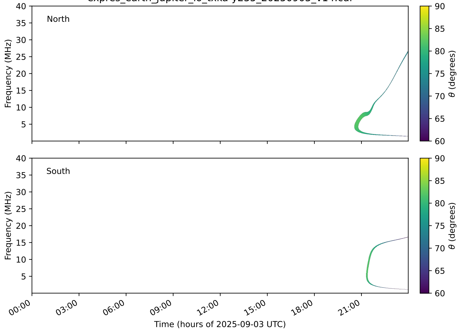
expres_earth_jupiter_io_txka-y235_20250903_v14.cdf
