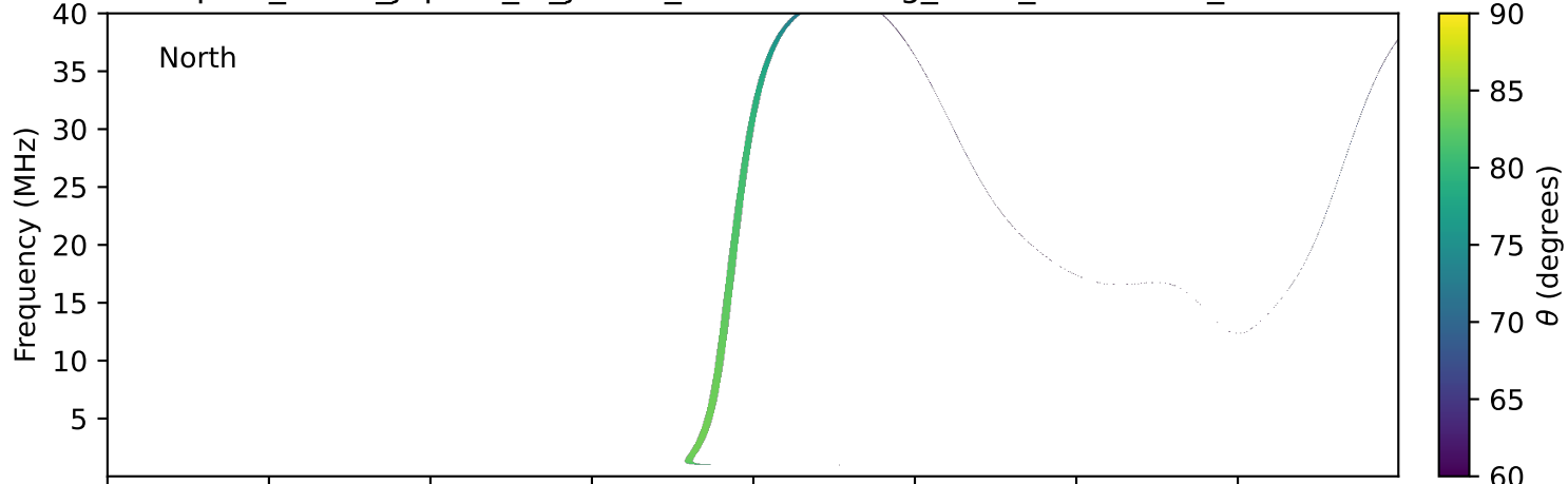
expres_earth_jupiter_io_jrm33_lossc-wid1deg_3kev_20250930_v11.cdf
