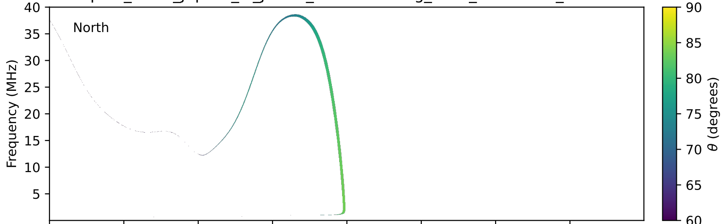
expres_earth_jupiter_io_jrm33_lossc-wid1deg_3kev_20250929_v11.cdf
