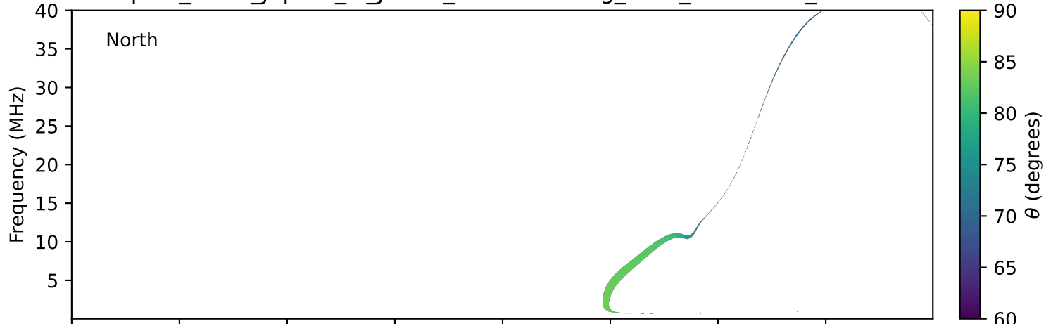
expres_earth_jupiter_io_jrm33_lossc-wid1deg_3kev_20250928_v11.cdf
