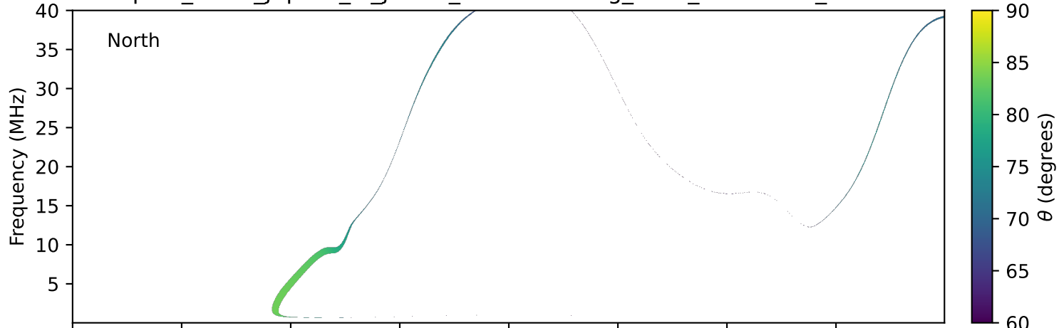
expres_earth_jupiter_io_jrm33_lossc-wid1deg_3kev_20250916_v11.cdf
