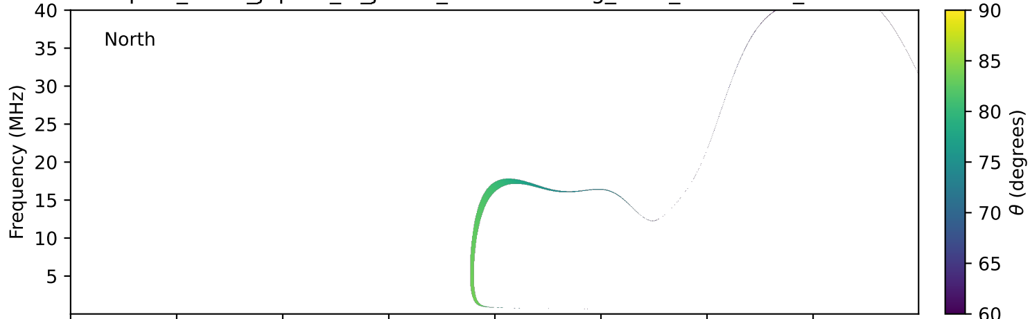
expres_earth_jupiter_io_jrm33_lossc-wid1deg_3kev_20250914_v11.cdf
