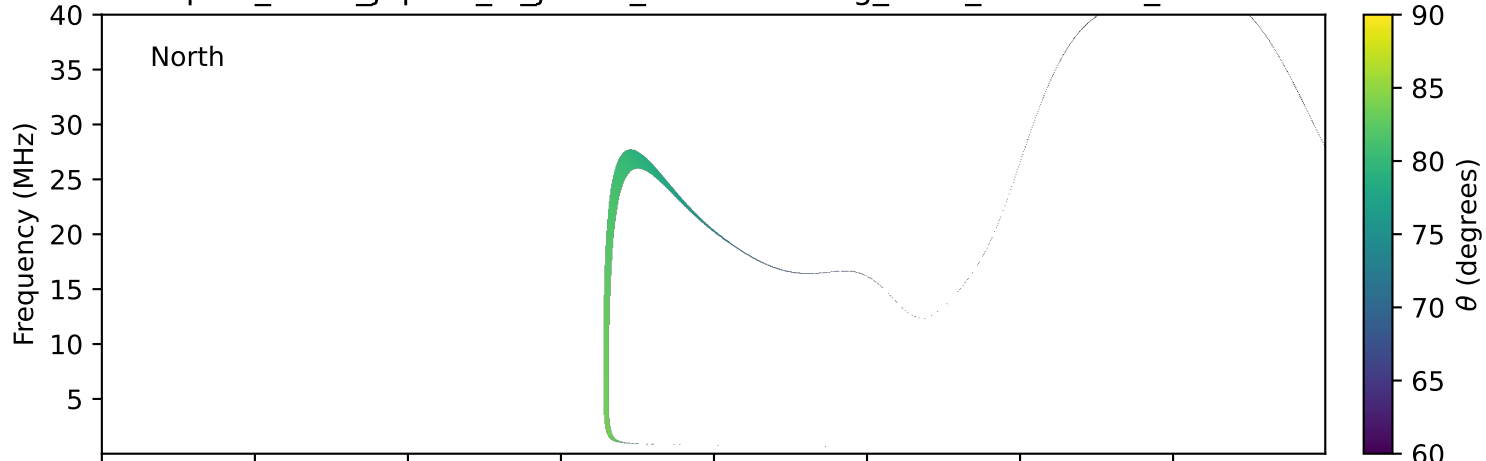
expres_earth_jupiter_io_jrm33_lossc-wid1deg_3kev_20250907_v11.cdf
