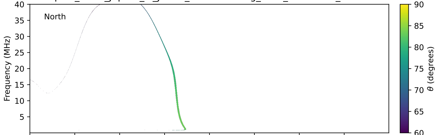
expres_earth_jupiter_io_jrm33_lossc-wid1deg_3kev_20250906_v11.cdf
