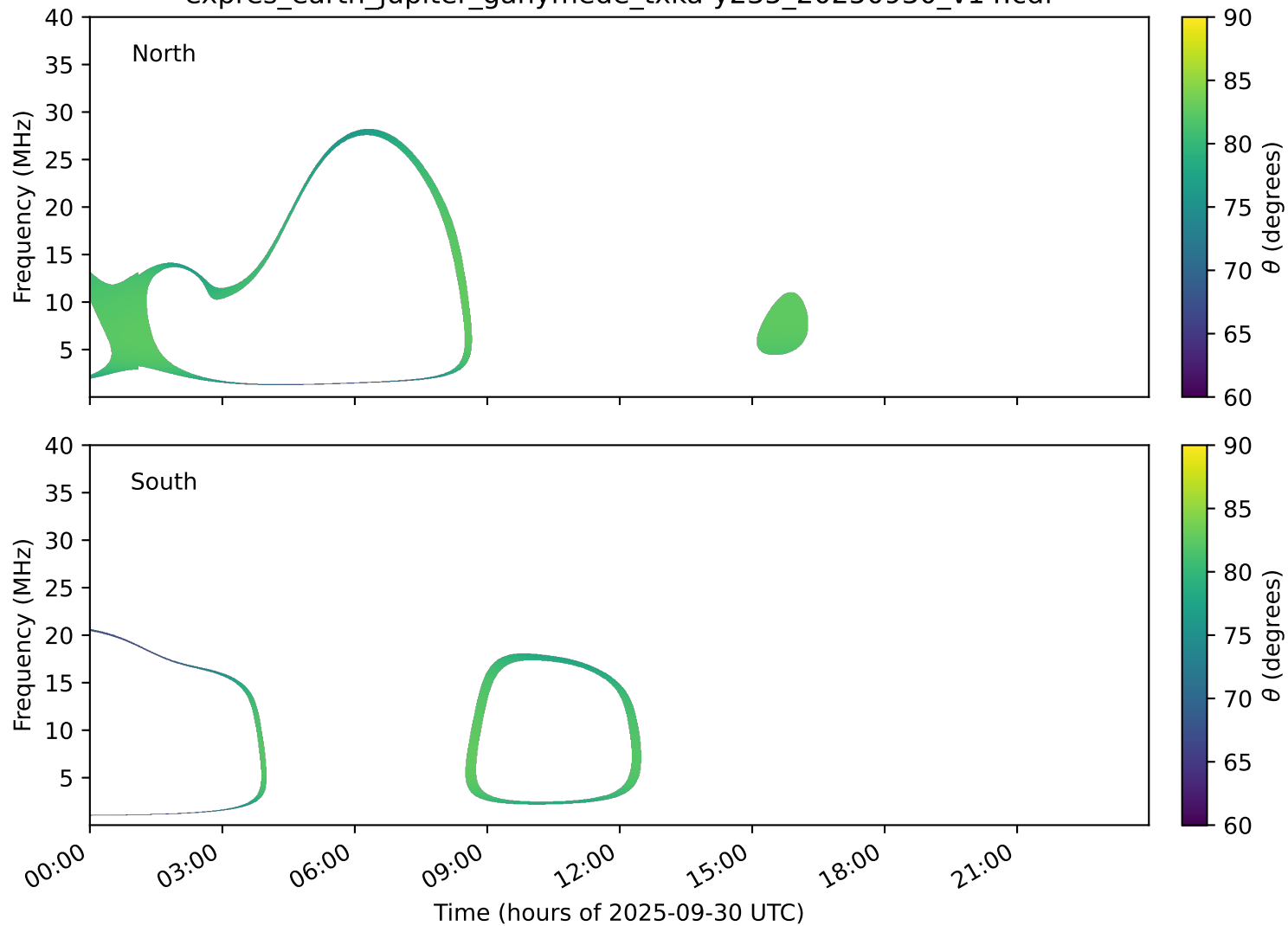
expres_earth_jupiter_ganymede_txka-y235_20250930_v14.cdf
