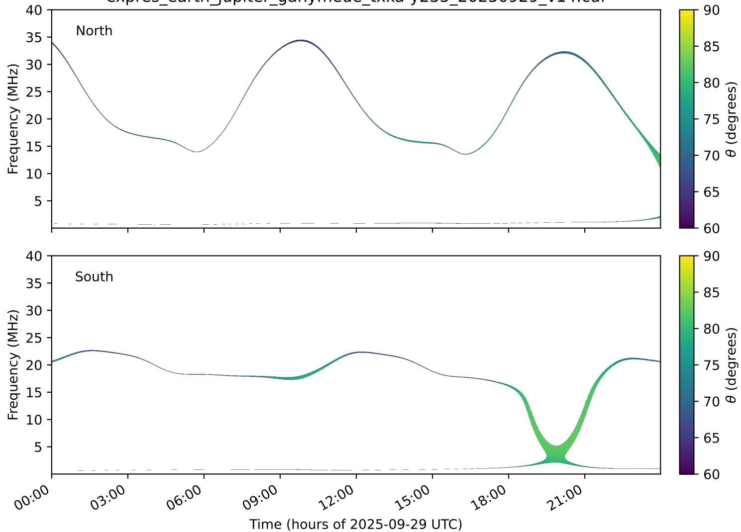
expres_earth_jupiter_ganymede_txka-y235_20250929_v14.cdf
