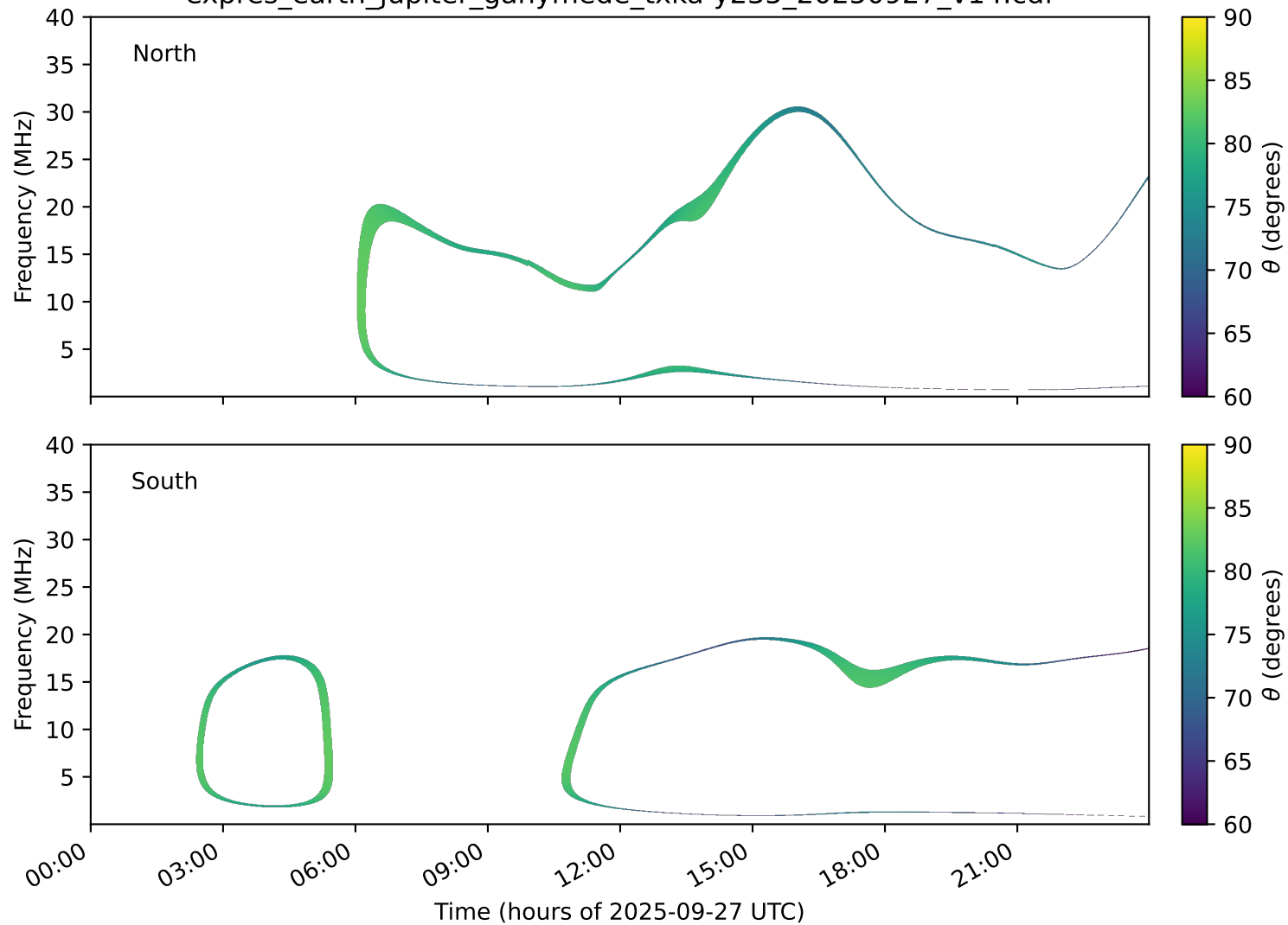
expres_earth_jupiter_ganymede_txka-y235_20250927_v14.cdf
