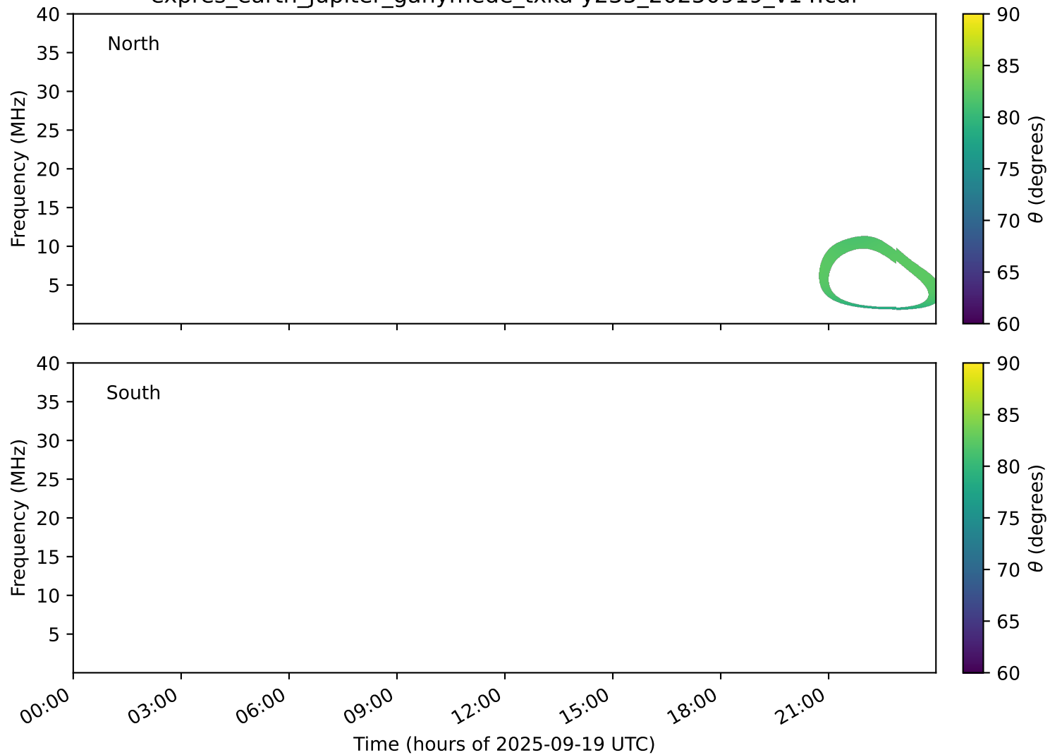
expres_earth_jupiter_ganymede_txka-y235_20250919_v14.cdf
