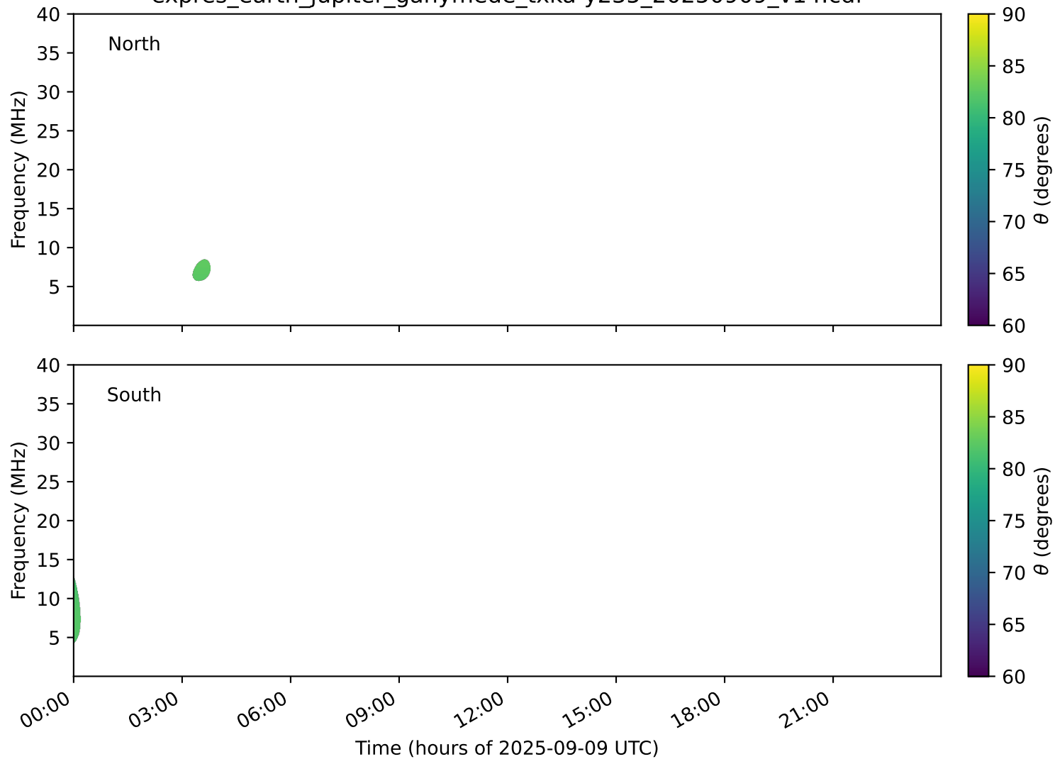
expres_earth_jupiter_ganymede_txka-y235_20250909_v14.cdf
