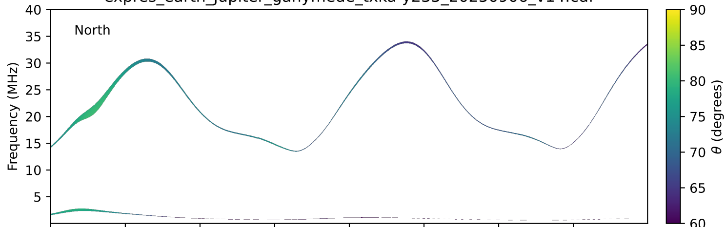
expres_earth_jupiter_ganymede_txka-y235_20250906_v14.cdf
