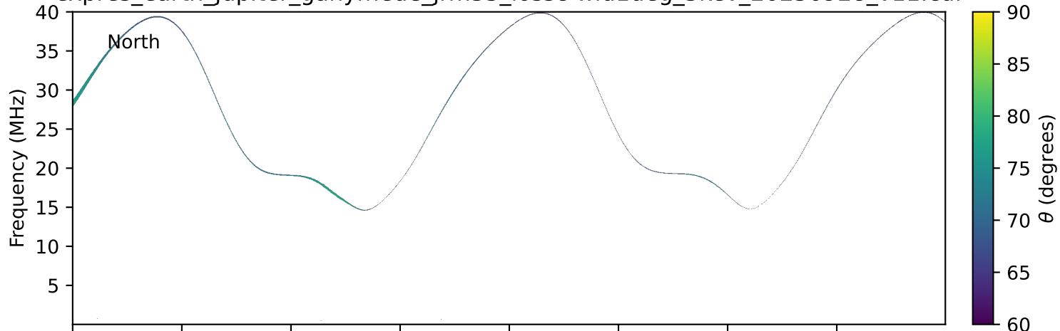
expres_earth_jupiter_ganymede_jrm33_lossc-wid1deg_3kev_20250928_v11.cdf
