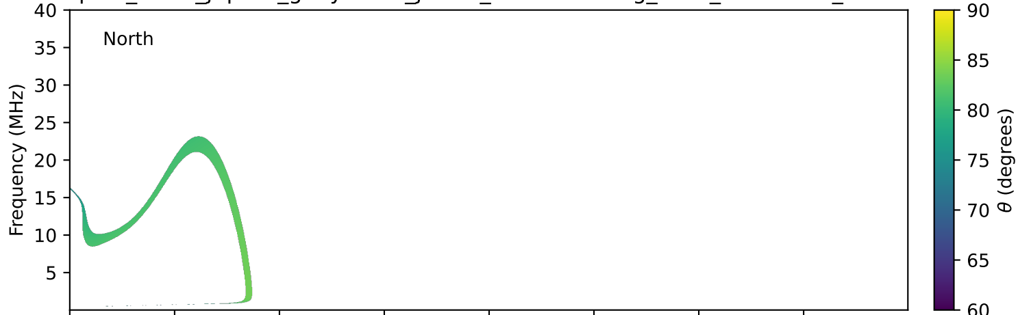
expres_earth_jupiter_ganymede_jrm33_lossc-wid1deg_3kev_20250909_v11.cdf
