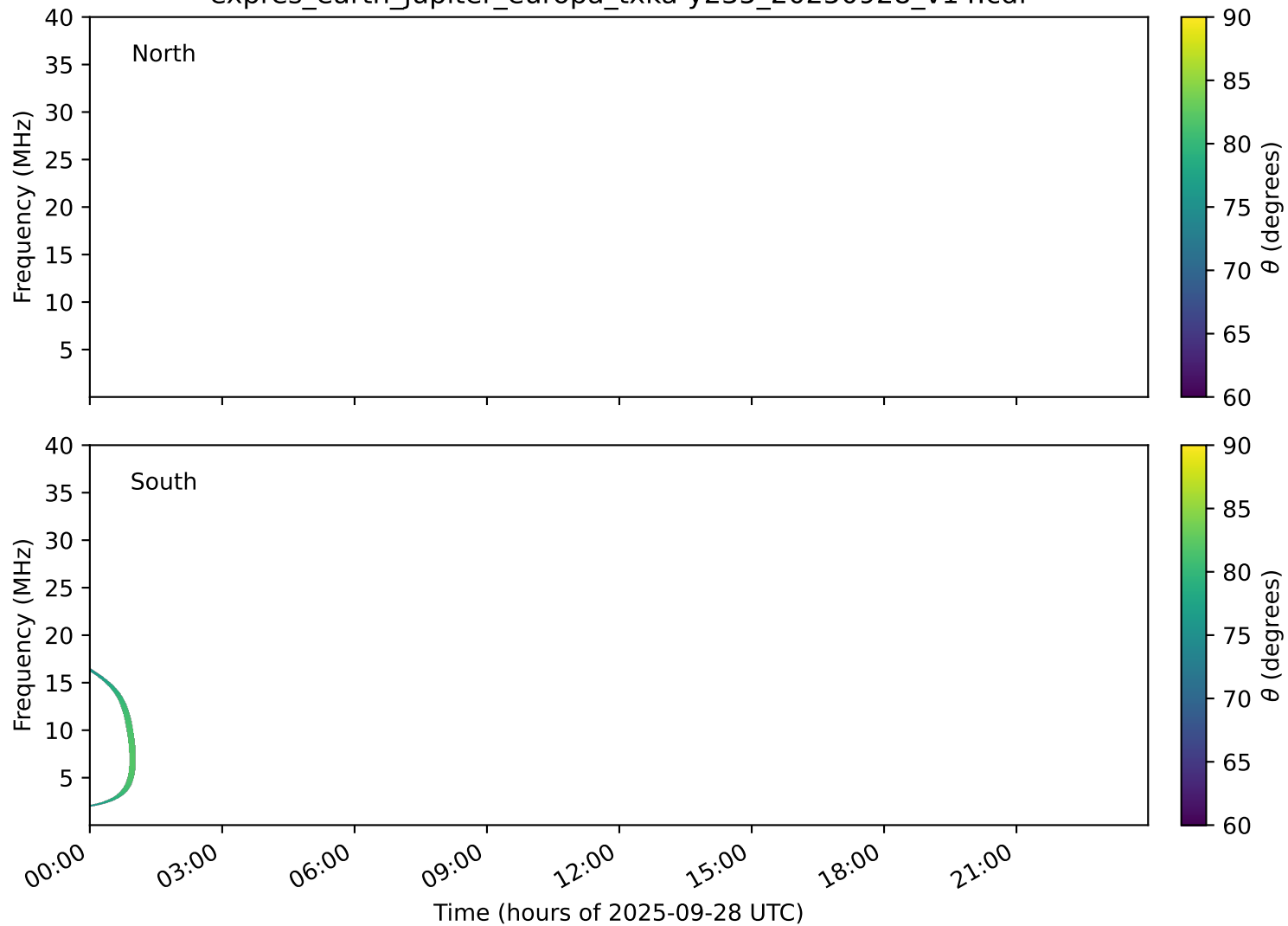
expres_earth_jupiter_europa_txka-y235_20250928_v14.cdf
