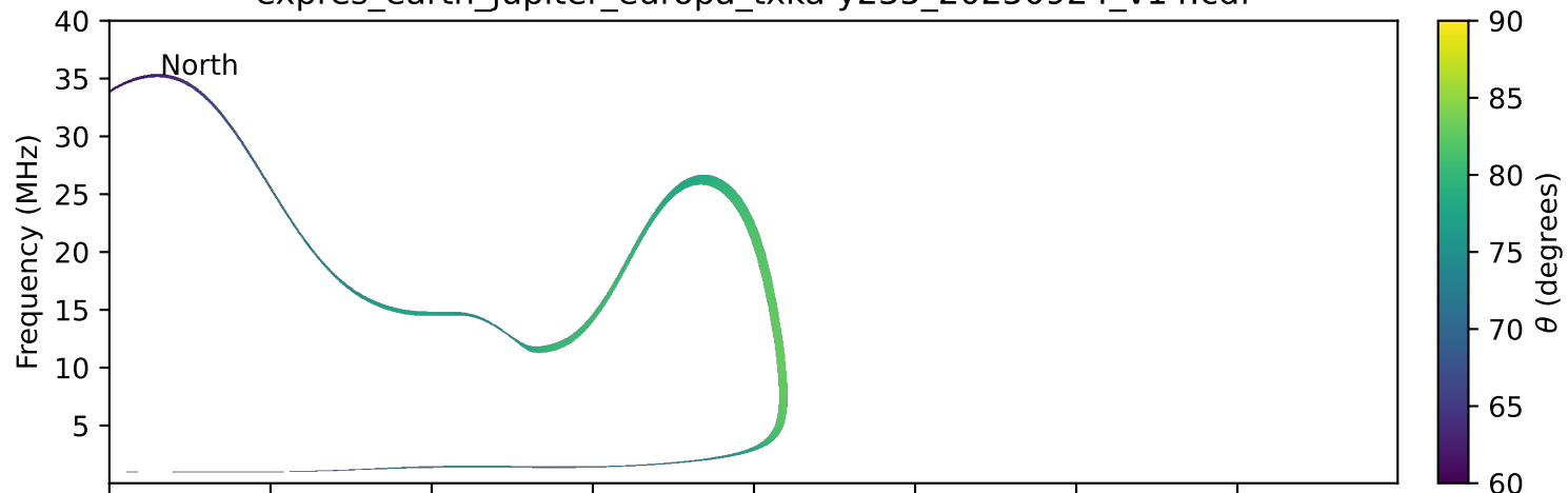
expres_earth_jupiter_europa_txka-y235_20250924_v14.cdf
