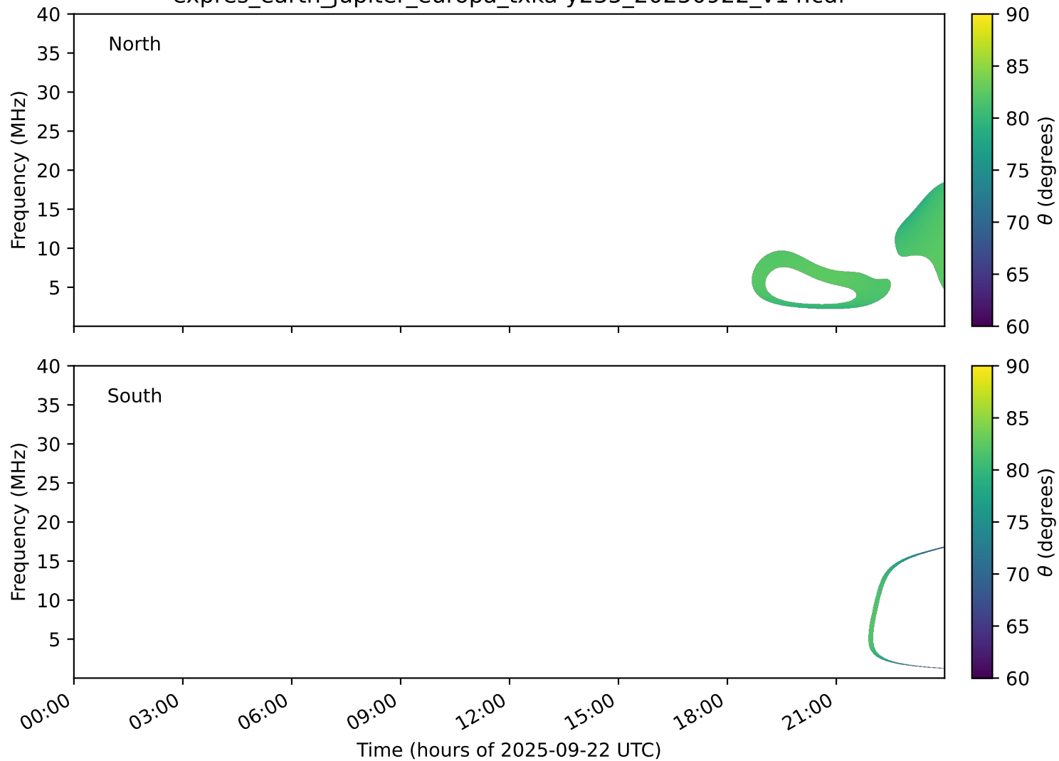
expres_earth_jupiter_europa_txka-y235_20250922_v14.cdf
