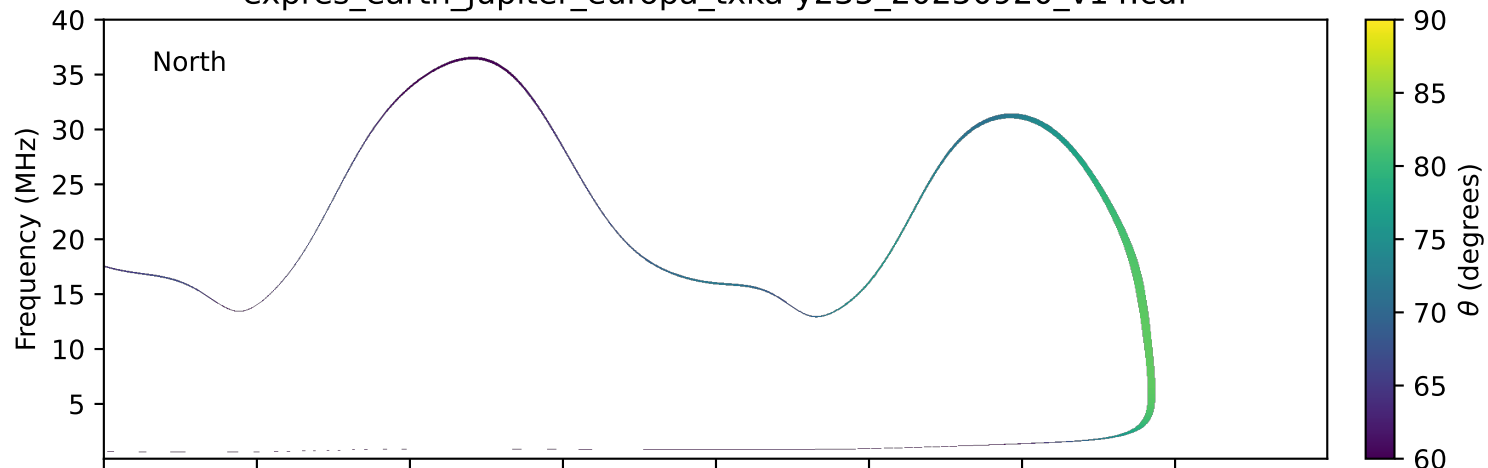
expres_earth_jupiter_europa_txka-y235_20250920_v14.cdf
