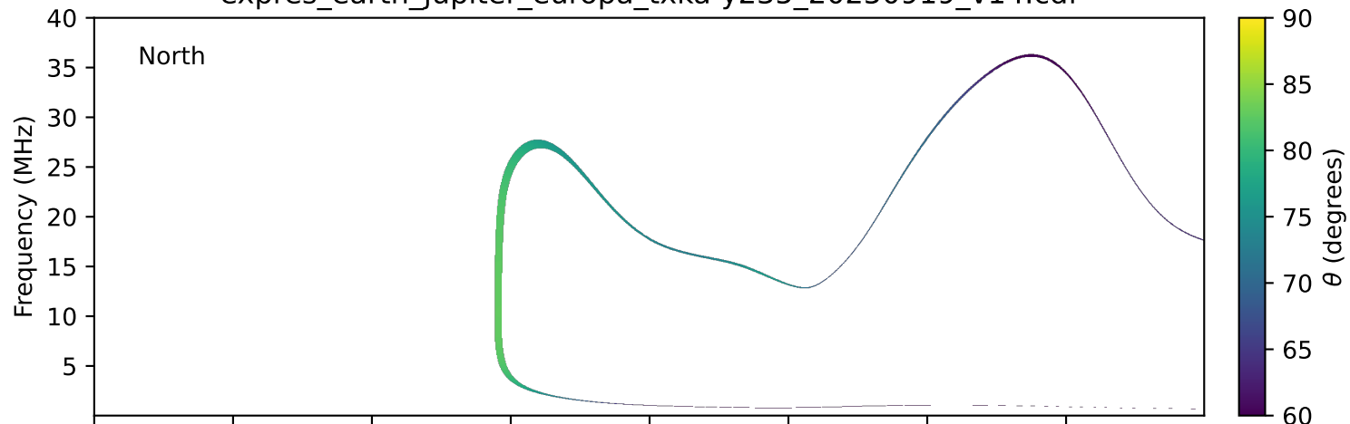
expres_earth_jupiter_europa_txka-y235_20250919_v14.cdf
