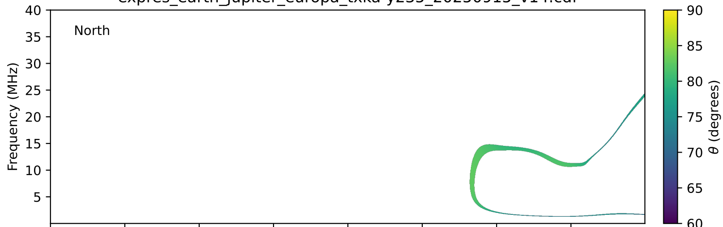
expres_earth_jupiter_europa_txka-y235_20250915_v14.cdf
