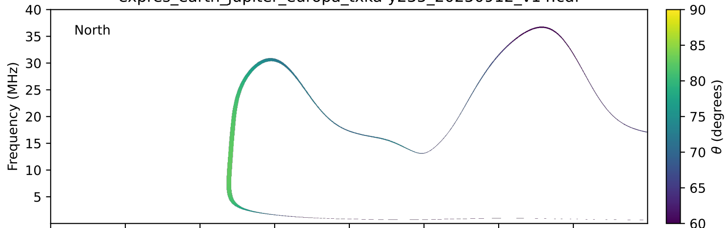
expres_earth_jupiter_europa_txka-y235_20250912_v14.cdf
