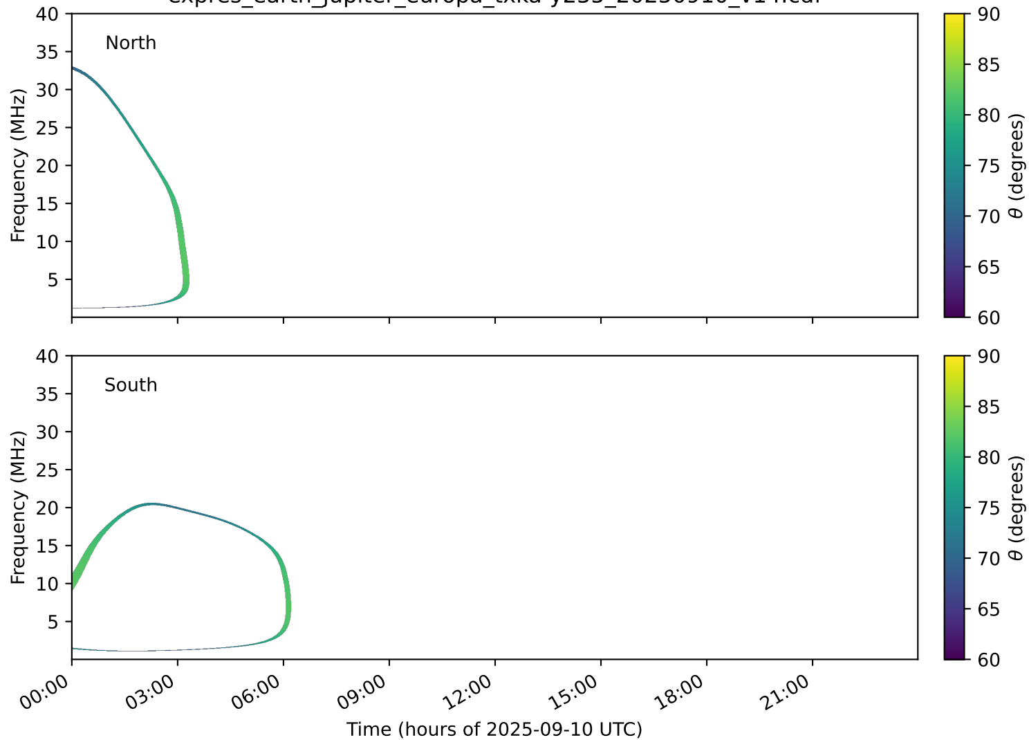
expres_earth_jupiter_europa_txka-y235_20250910_v14.cdf
