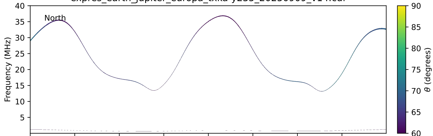
expres_earth_jupiter_europa_txka-y235_20250909_v14.cdf
