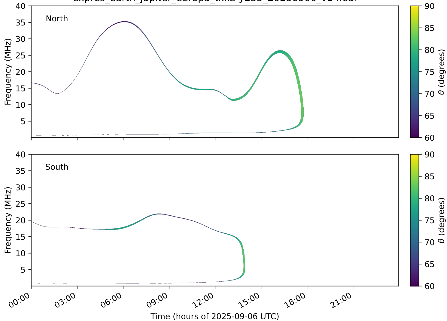
expres_earth_jupiter_europa_txka-y235_20250906_v14.cdf
