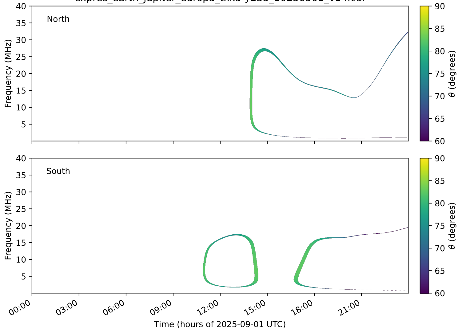
expres_earth_jupiter_europa_txka-y235_20250901_v14.cdf
