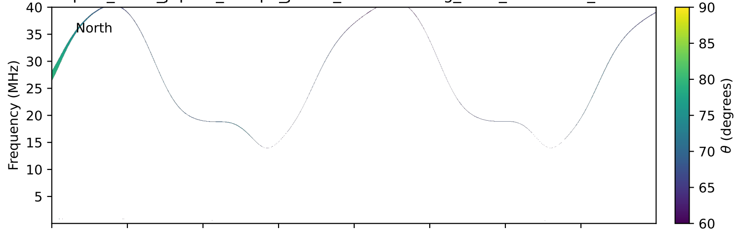
expres_earth_jupiter_europa_jrm33_lossc-wid1deg_3kev_20250916_v11.cdf
