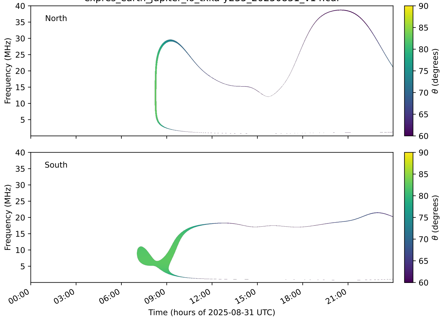
expres_earth_jupiter_io_txka-y235_20250831_v14.cdf
