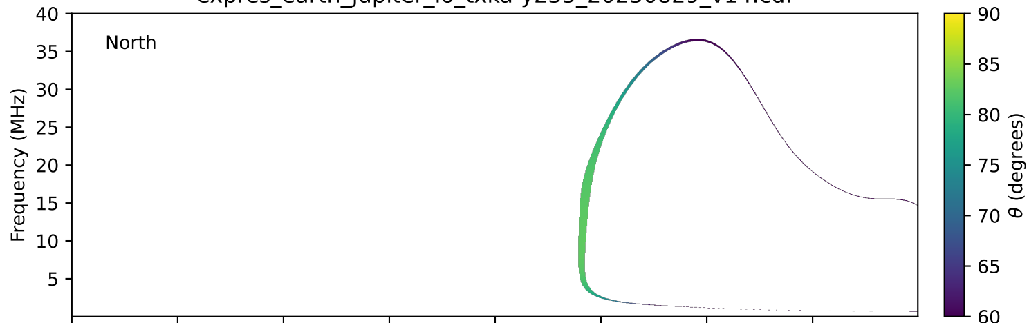
expres_earth_jupiter_io_txka-y235_20250829_v14.cdf
