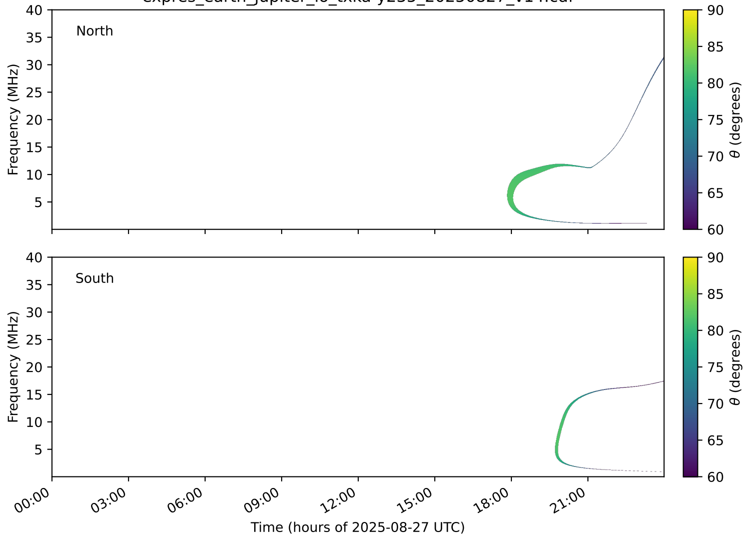
expres_earth_jupiter_io_txka-y235_20250827_v14.cdf
