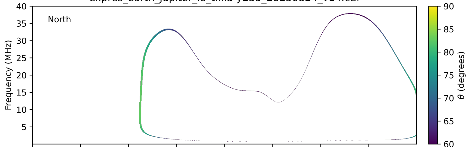
expres_earth_jupiter_io_txka-y235_20250824_v14.cdf
