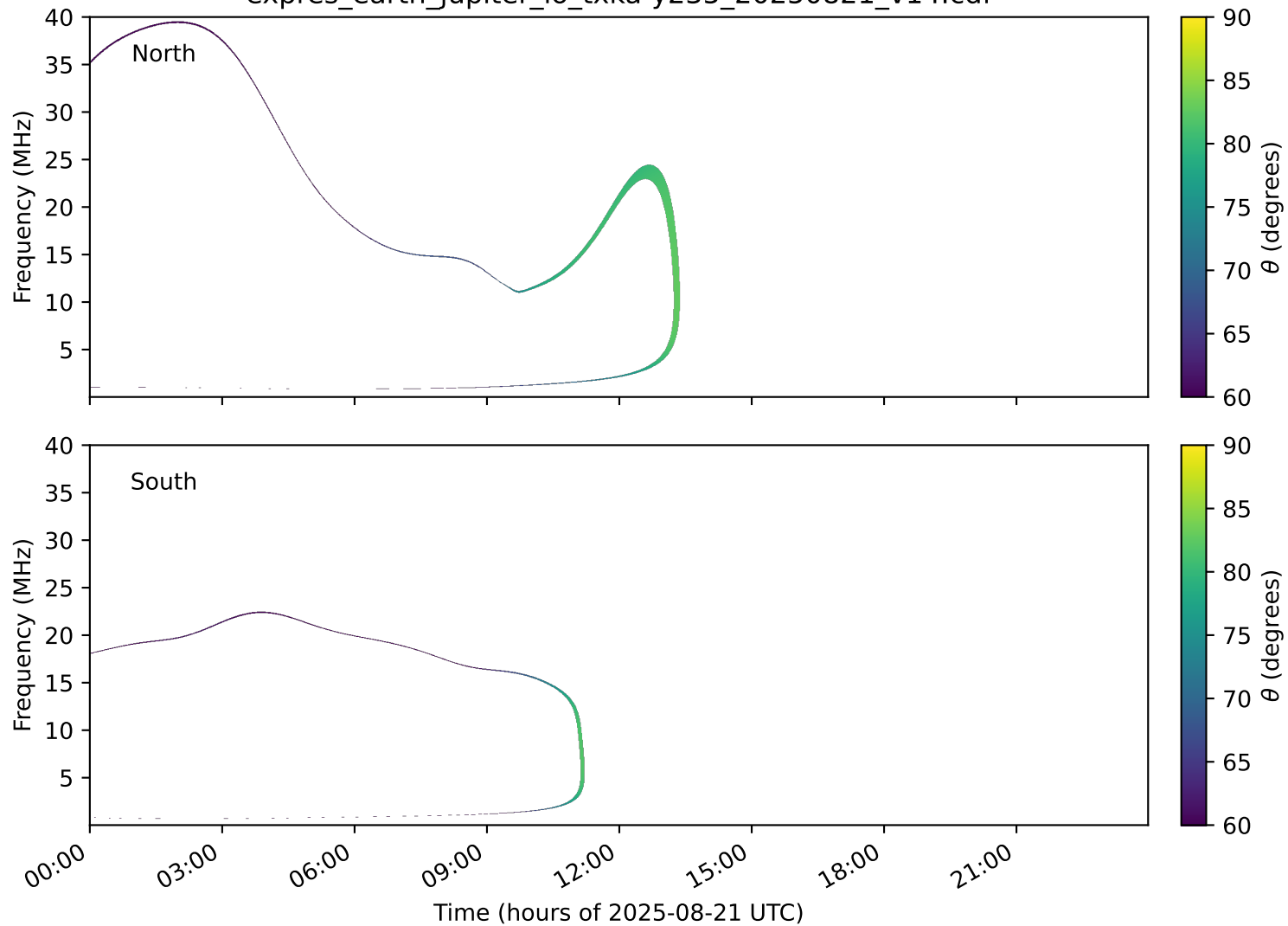
expres_earth_jupiter_io_txka-y235_20250821_v14.cdf
