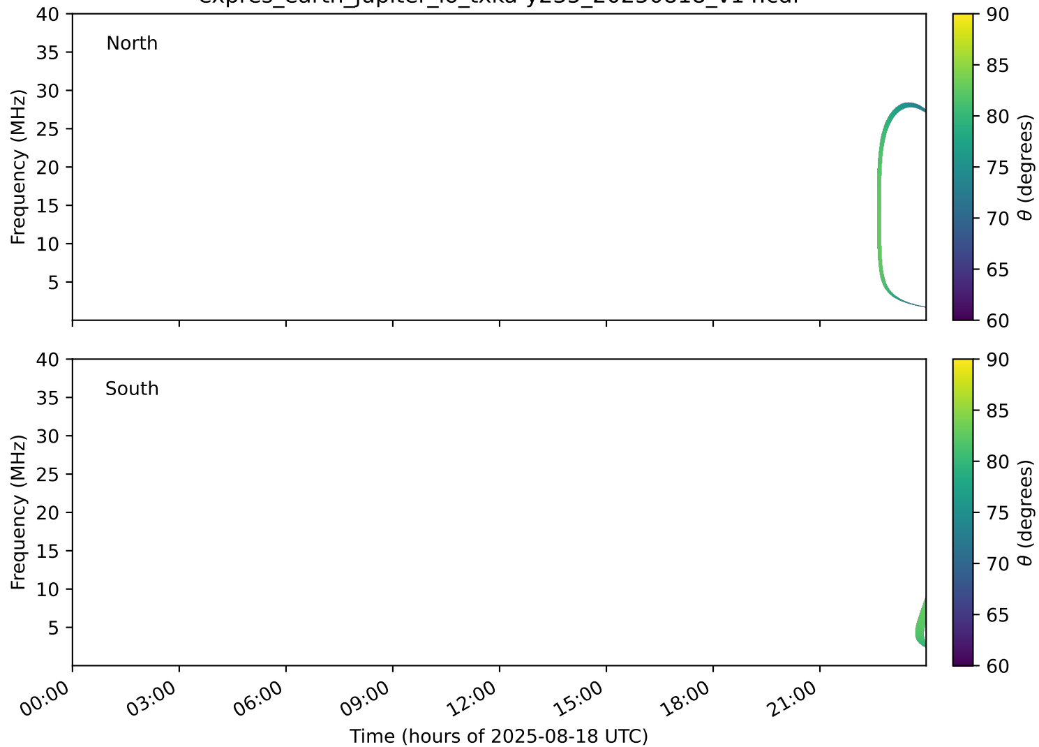
expres_earth_jupiter_io_txka-y235_20250818_v14.cdf
