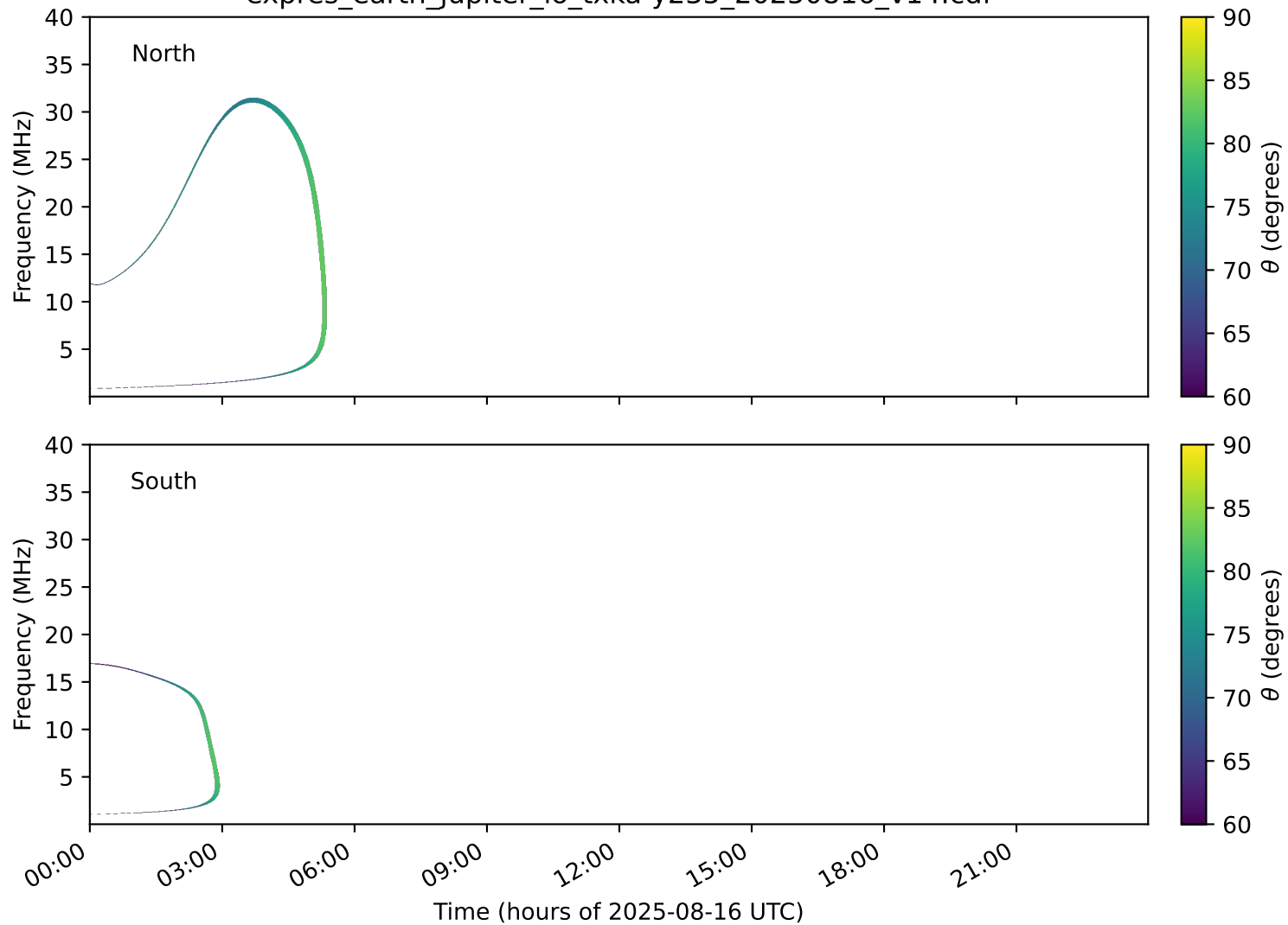
expres_earth_jupiter_io_txka-y235_20250816_v14.cdf
