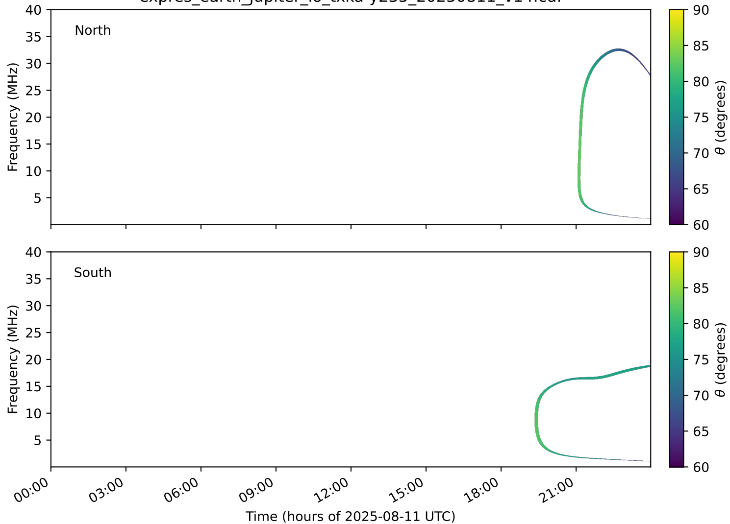
expres_earth_jupiter_io_txka-y235_20250811_v14.cdf
