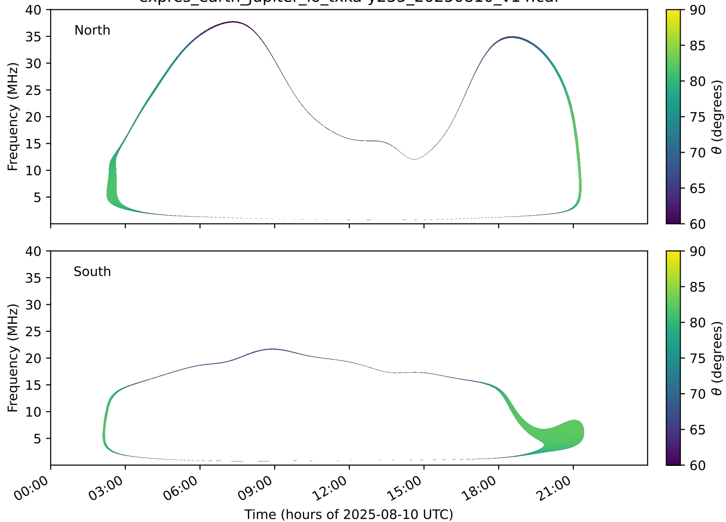
expres_earth_jupiter_io_txka-y235_20250810_v14.cdf
