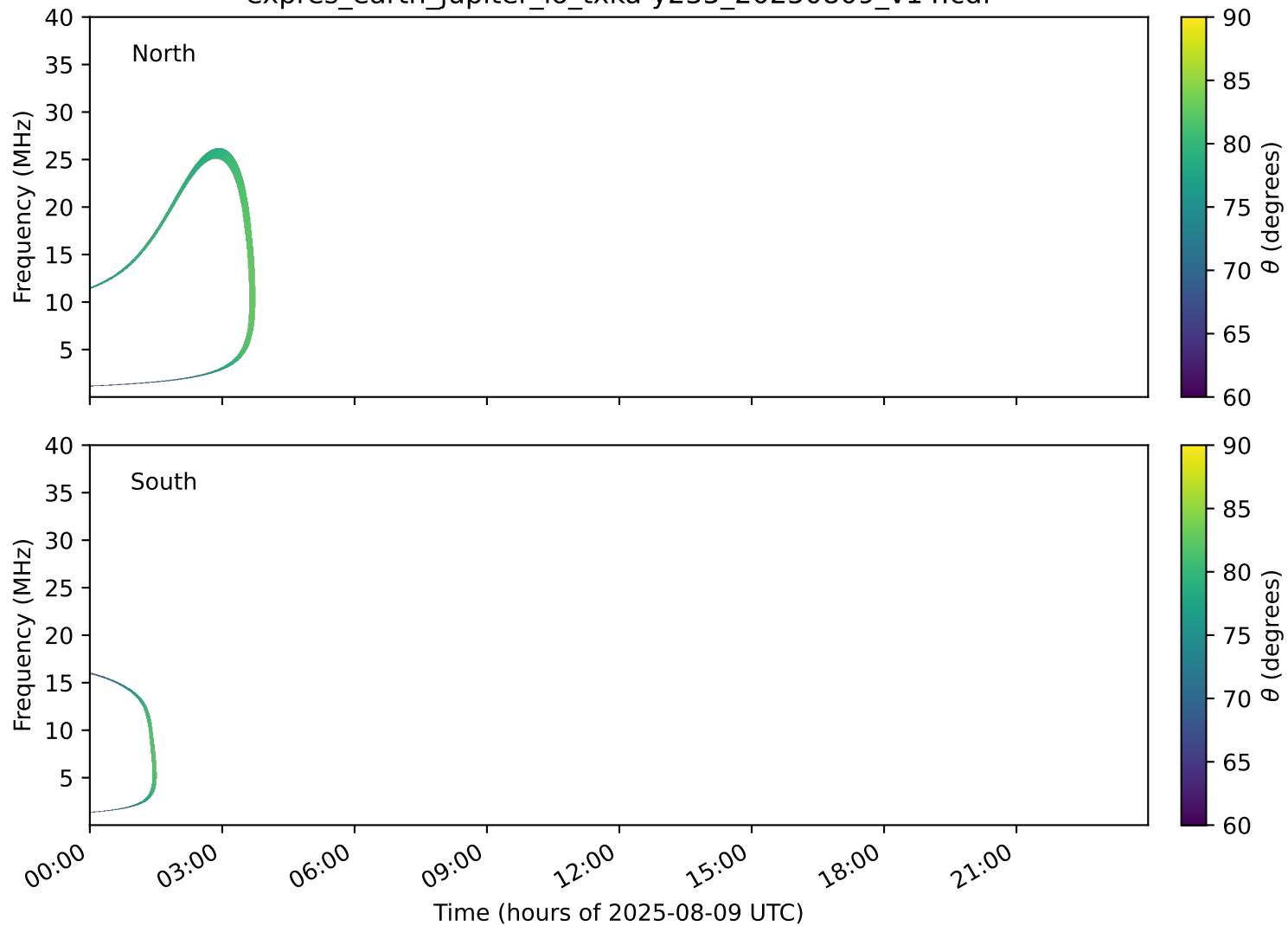
expres_earth_jupiter_io_txka-y235_20250809_v14.cdf
